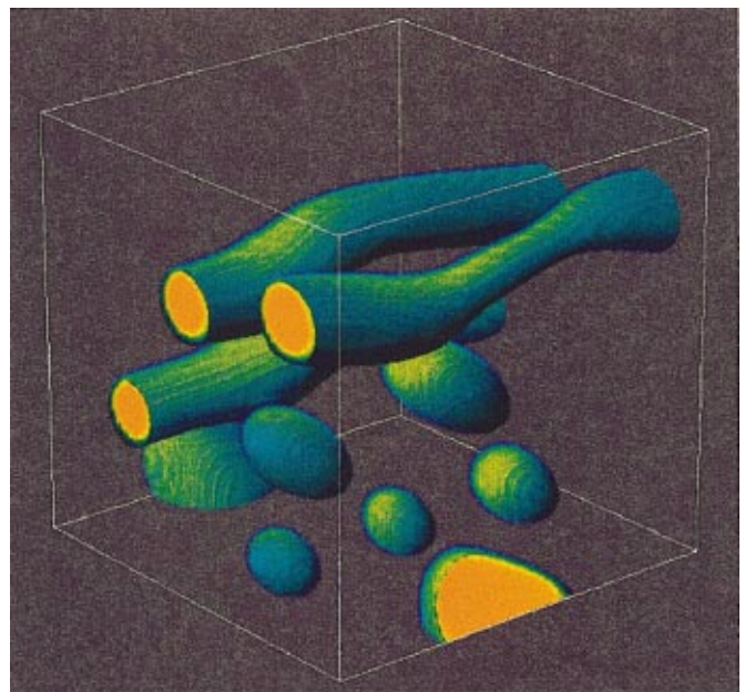
FIG. 17. (Color) Late-stage off-critical (15-85) phase separation ( \bar{t}=56.8 ). Droplets shown in Fig. 15 reconnect into stringlike structures that appear to persist and coarsen in cross-sectional dimension with time. The strings in Fig. 17 are contrasted with the “stringslike” structures near the mixture surface in Fig. 14, representative of a critical composition fluid mixture.
